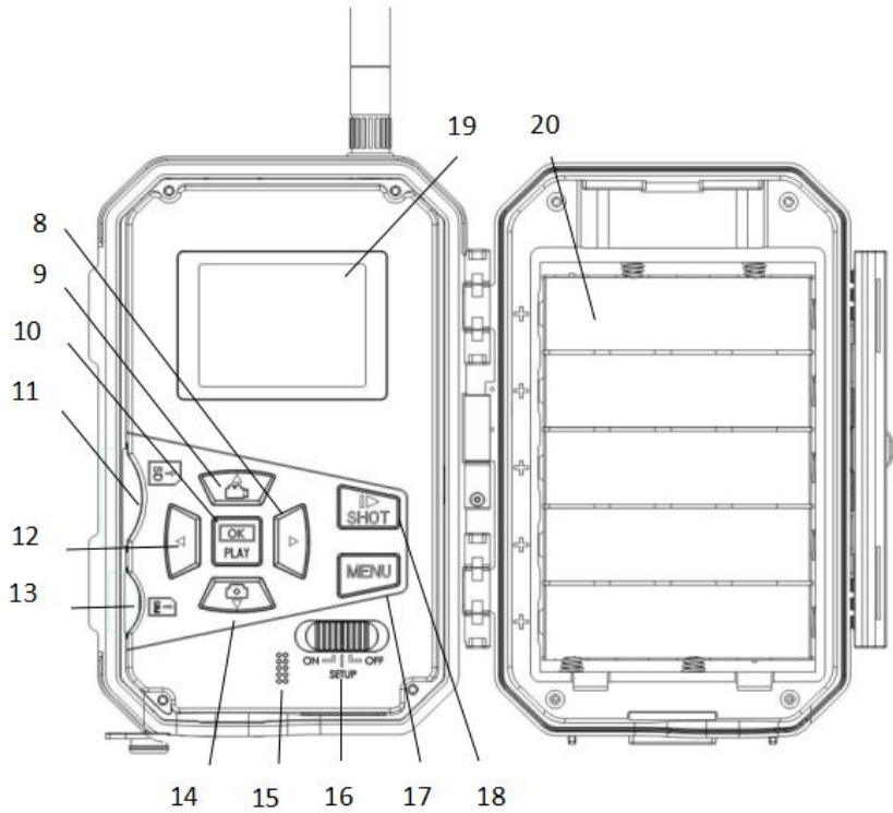
Fig. 2: Inner Panel View
